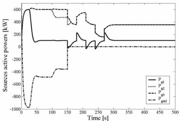
Fig. 14. GS and grid active powers.
