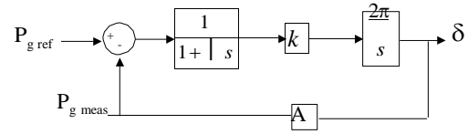
Fig. 5. Generating system delivered active power closed loop control.
