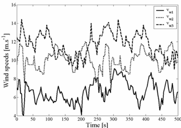
Fig. 12. Wind speed evolutions.
