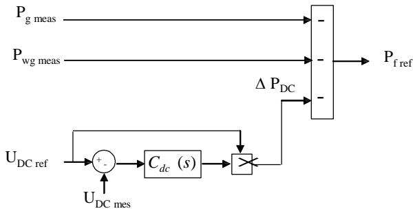
Fig. 8. Power reference of the storage system determination.
