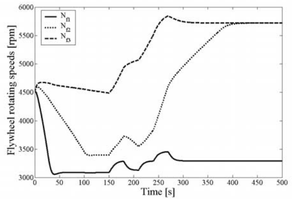
Fig. 16. Flywheel rotating speeds.
