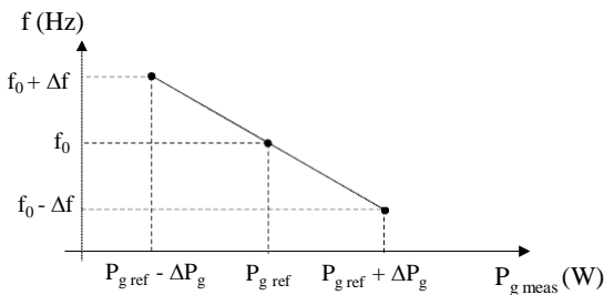
Fig. 4. Frequency droop.
