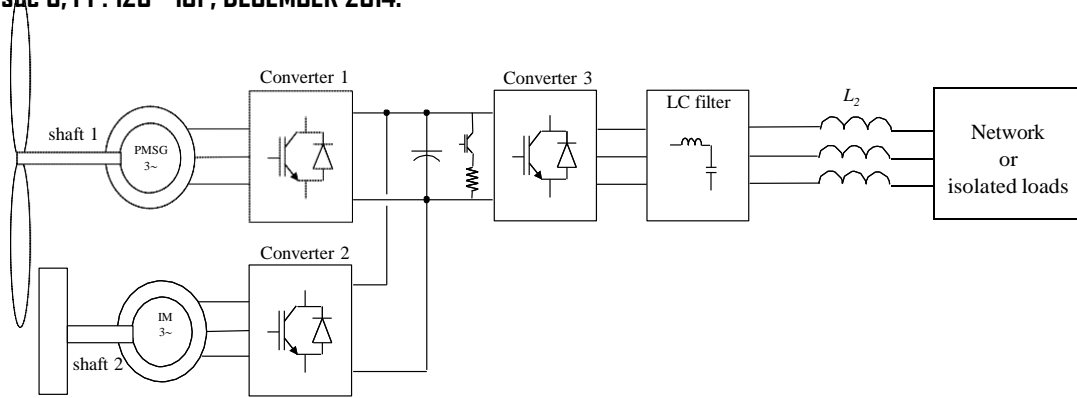
Fig. 1. Scheme of a generating system.
