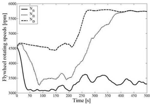
Fig. 22. Flywheel rotating speeds.
