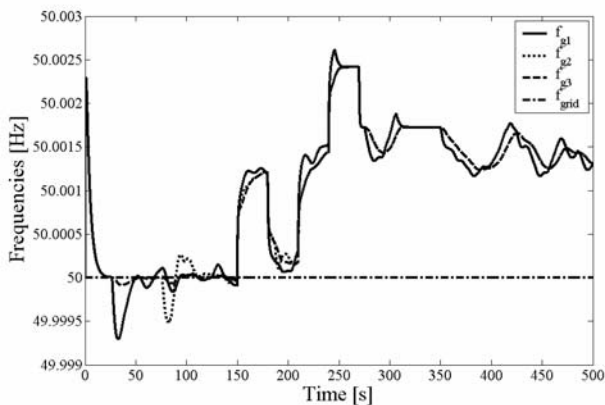
Fig. 24. Generating system reference and grid frequencies.
